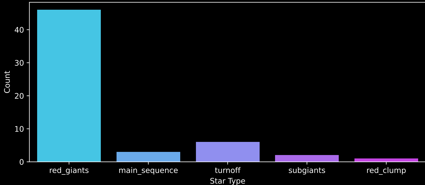
APOGEE DR17 Field: [276-34-O] Count plot of Star Type
