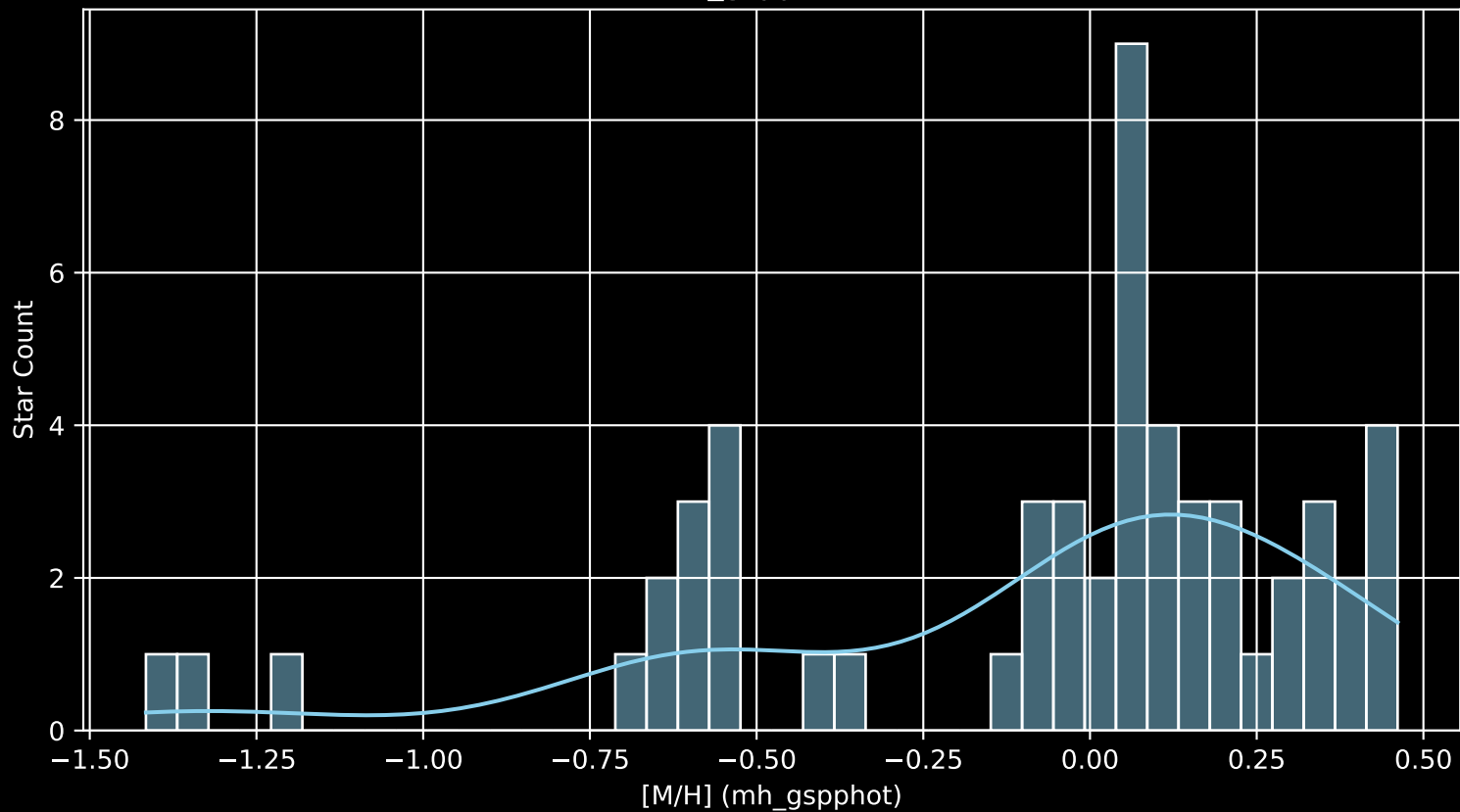
APOGEE DR17 Field: [276-34-O [M/H] (mh_gspphot) (n= 55)
