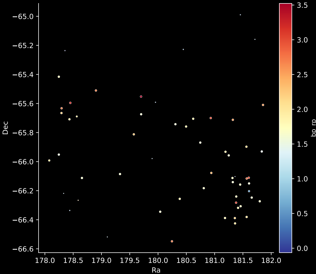
APOGEE DR17 Field: [276-34-O] Stars: 58
