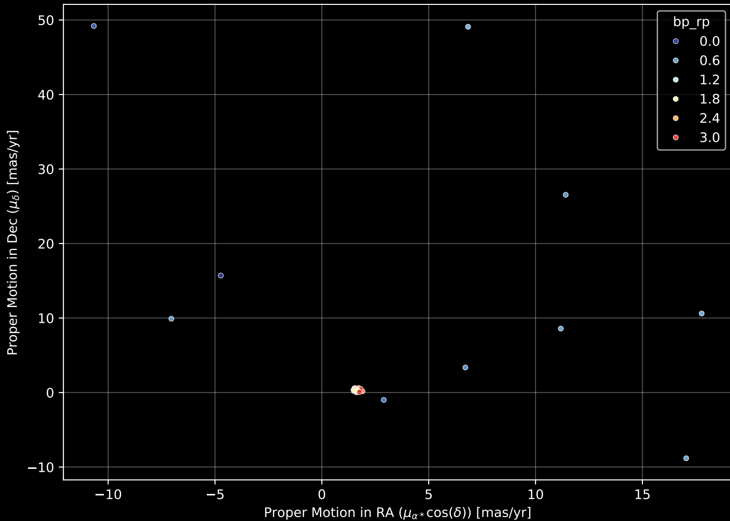
APOGEE DR17 Field: [276-34-O] Proper Motion Diagram (n= 58)
