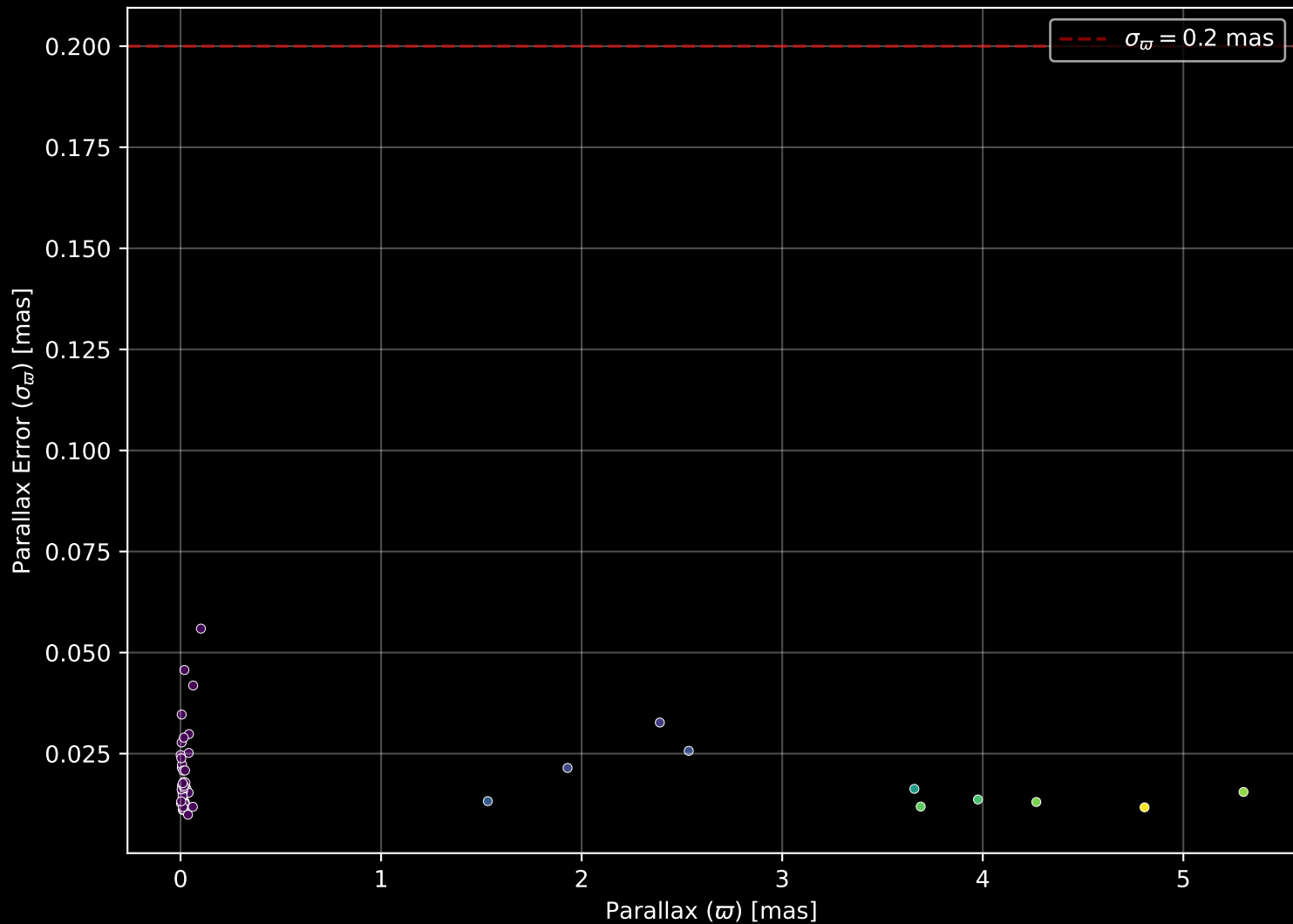
APOGEE DR17 Field: [276-34-O] Parallax Quality (n= 58)
