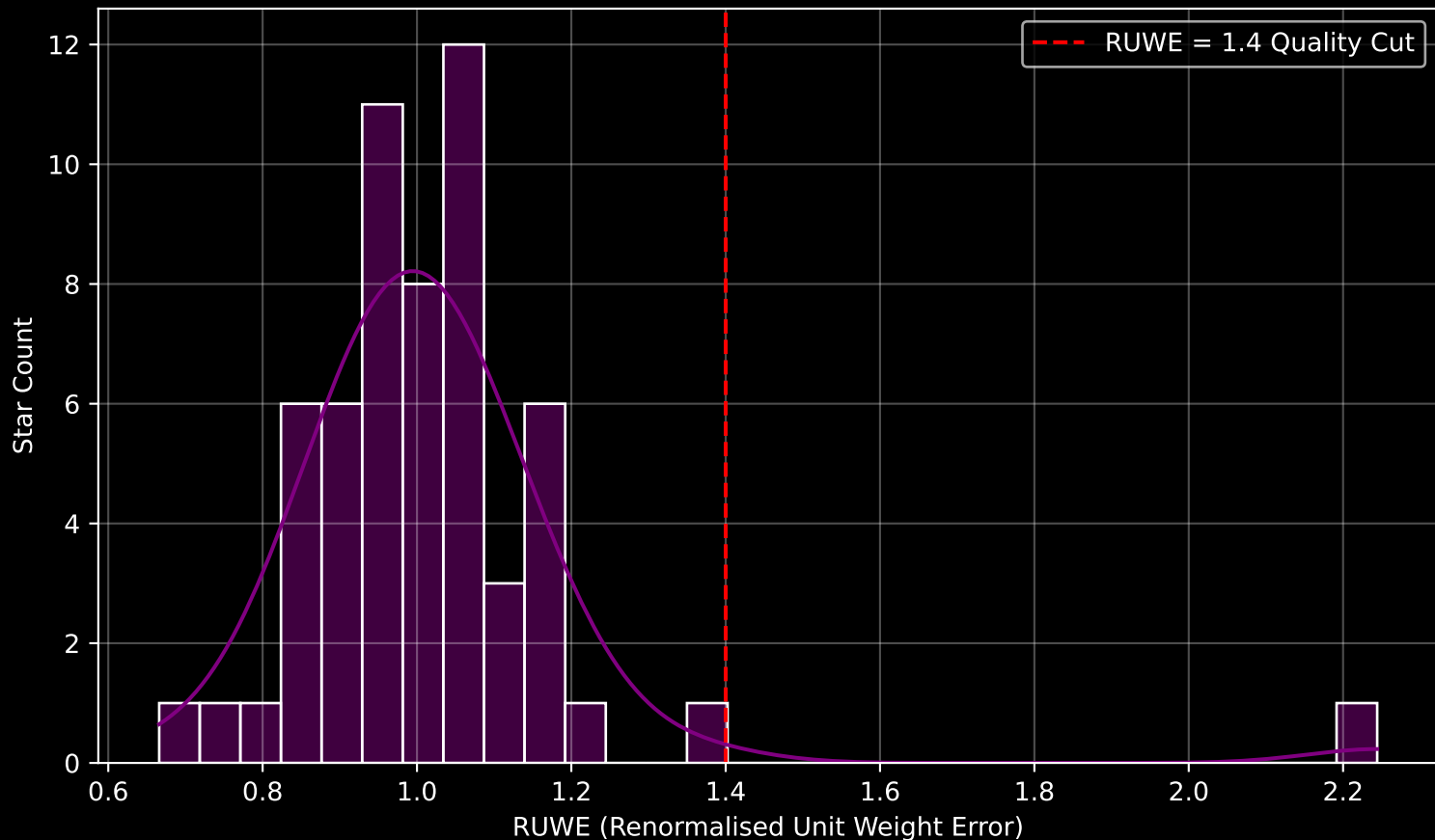
GAPOGEE DR17 Field [276-34-O] RUWE Distribution (n= 58)
