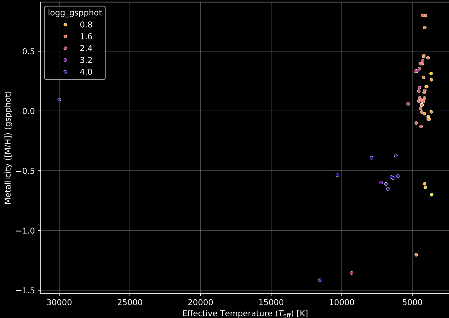
APOGEE DR17 Field: [276-34-O] Stellar Population Parameters (n= 58)
